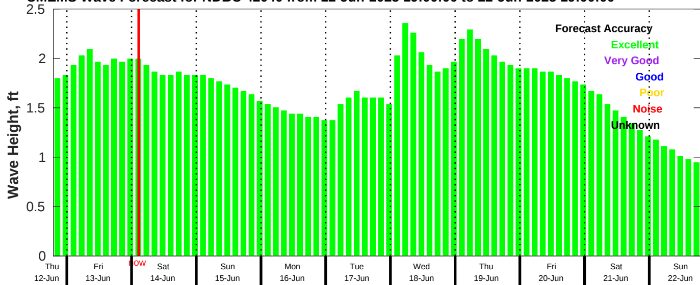
CMEMS Wave Forecast for NDBC 42040 from 12-Jun-2025 19:00:00 to 22-Jun-2025 19:00:00
