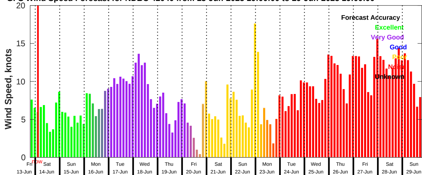
GFS Wind Speed Forecast for NDBC 42040 from 13-Jun-2025 19:00:00 to 29-Jun-2025 19:00:00
