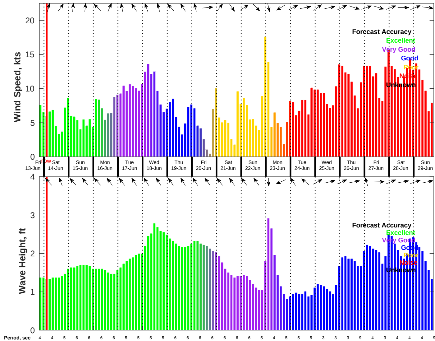
Wind & Wave Forecast for NDBC 42040 from 13-Jun-2025 19:00:00 to 29-Jun-2025 19:00:00
