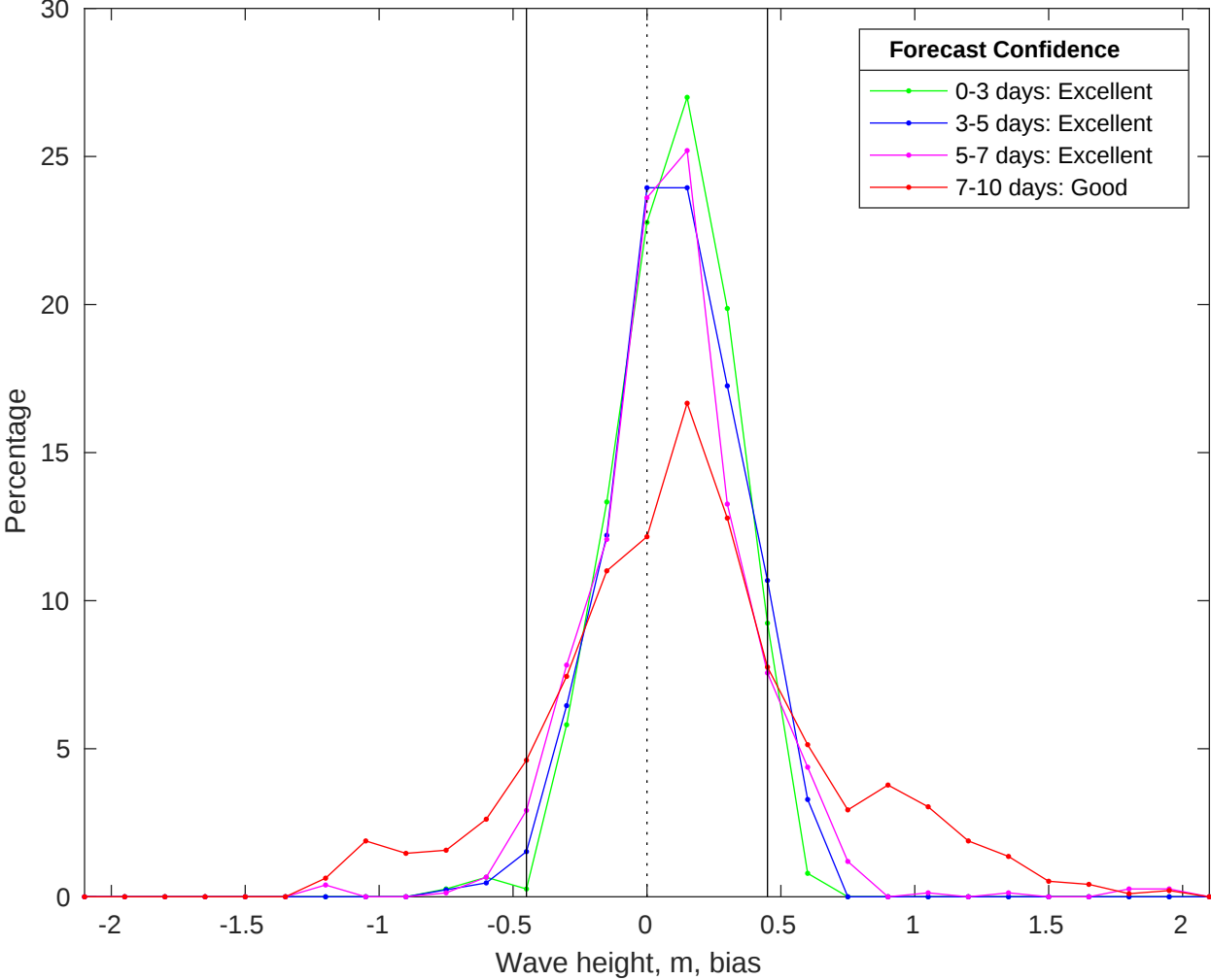
NDBC 46011 vs CMEMS Waves Bias Histogram: 14-Jun-2025
