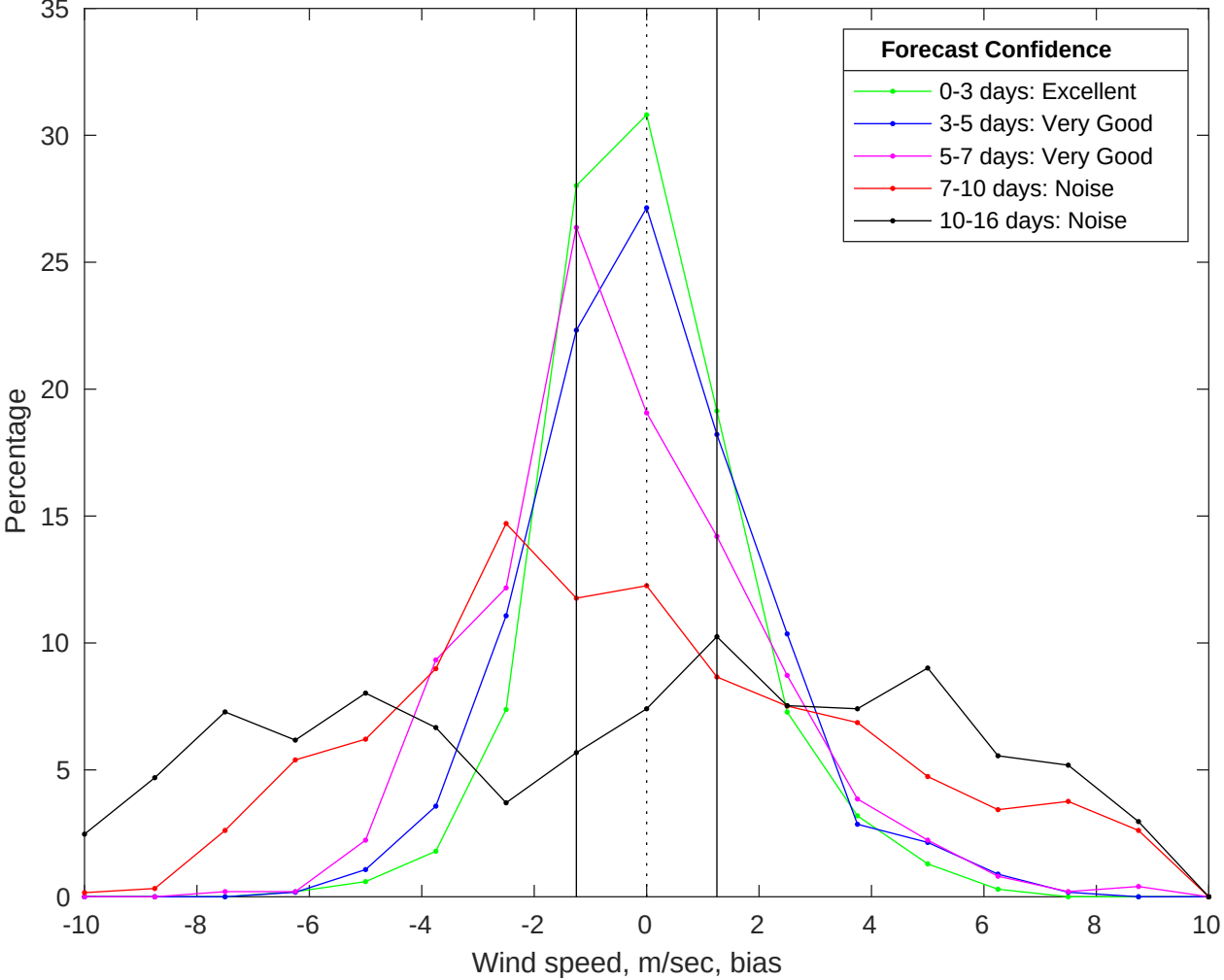
NDBC 46011 vs GFS Winds Bias Histogram: 14-Jun-2025
