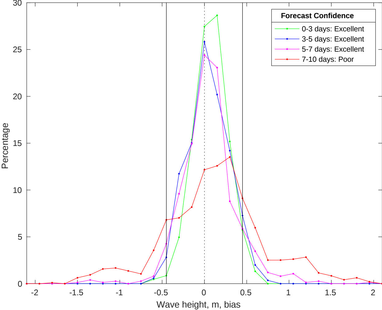
NDBC 46028 vs CMEMS Waves Bias Histogram: 14-Jun-2025
