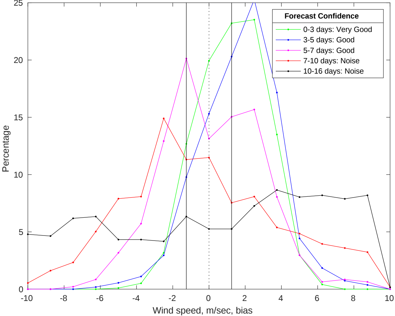
NDBC 46028 vs GFS Winds Bias Histogram: 14-Jun-2025
