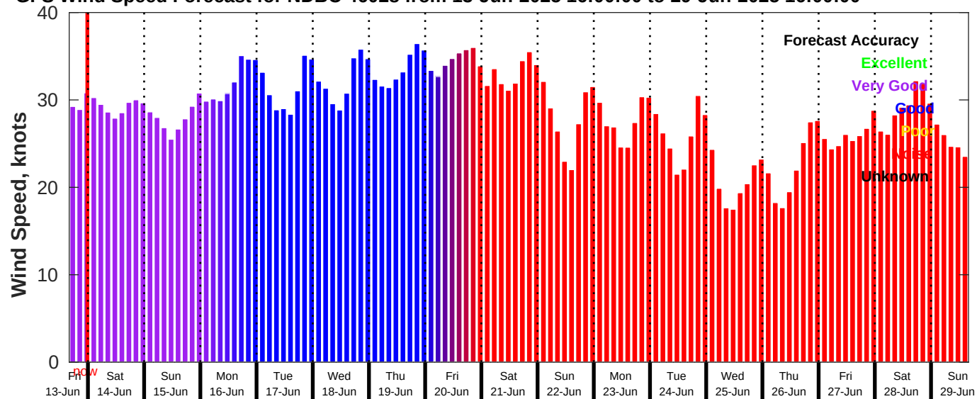
GFS Wind Speed Forecast for NDBC 46028 from 13-Jun-2025 16:00:00 to 29-Jun-2025 16:00:00
