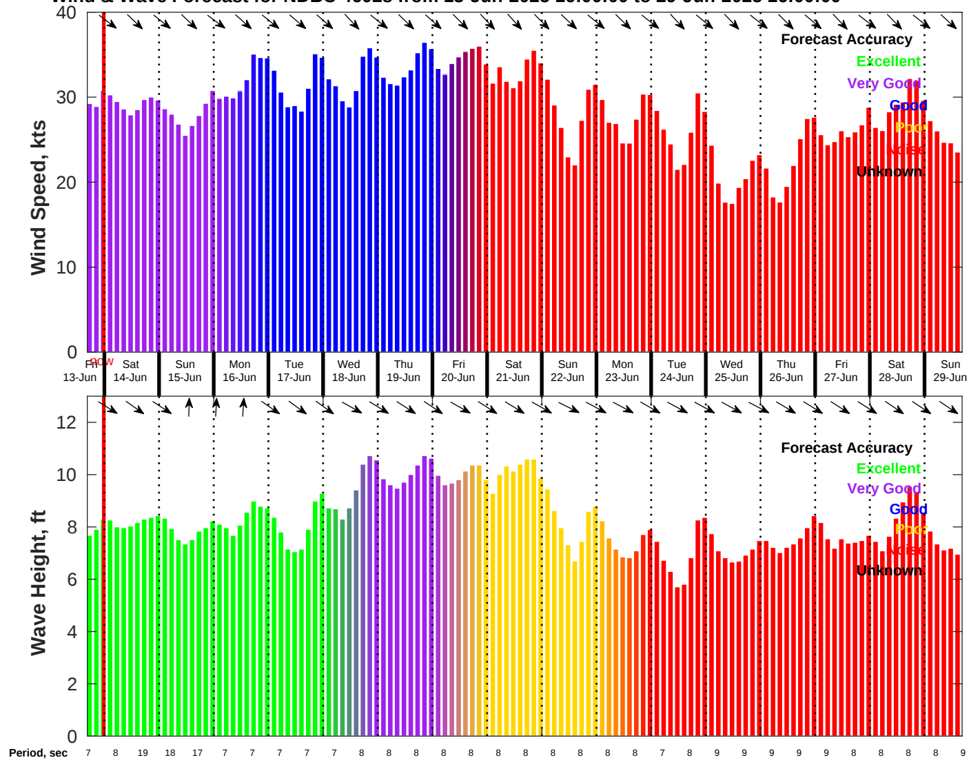
Wind & Wave Forecast for NDBC 46028 from 13-Jun-2025 16:00:00 to 29-Jun-2025 16:00:00
