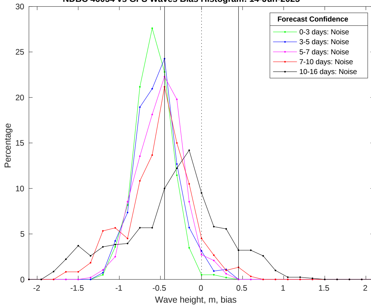
NDBC 46054 vs GFS Waves Bias Histogram: 14-Jun-2025
