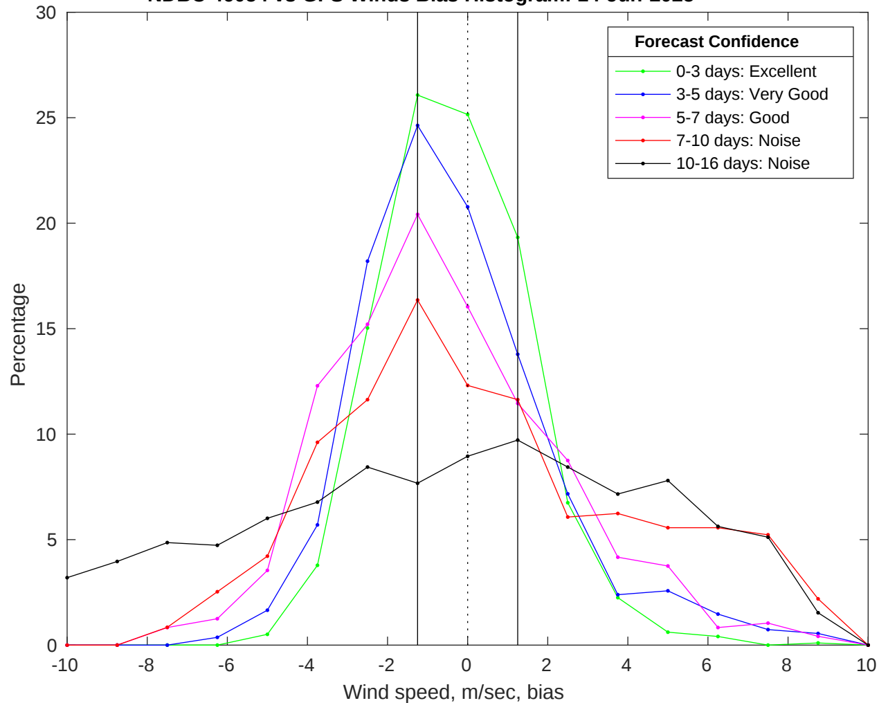
NDBC 46054 vs GFS Winds Bias Histogram: 14-Jun-2025
