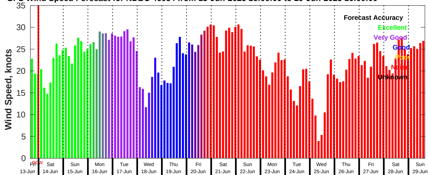
GFS Wind Speed Forecast for NDBC 46054 from 13-Jun-2025 16:00:00 to 29-Jun-2025 16:00:00
