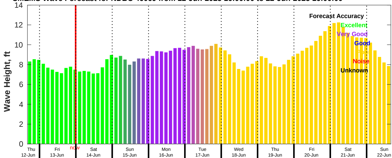
CMEMS Wave Forecast for NDBC 46069 from 12-Jun-2025 16:00:00 to 22-Jun-2025 16:00:00
