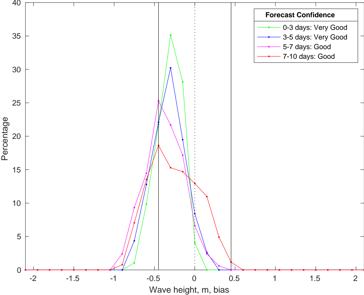
NDBC 51209 vs CMEMS Waves Bias Histogram: 14-Jun-2025
