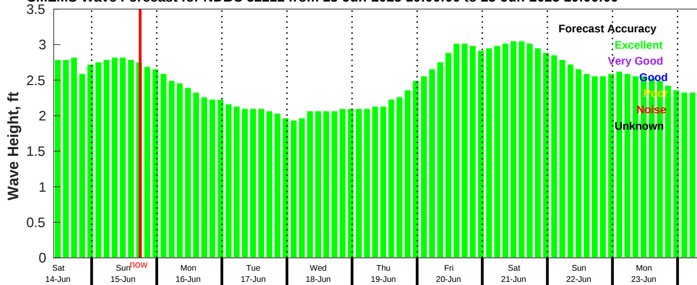
CMEMS Wave Forecast for NDBC 52211 from 13-Jun-2025 10:00:00 to 23-Jun-2025 10:00:00
