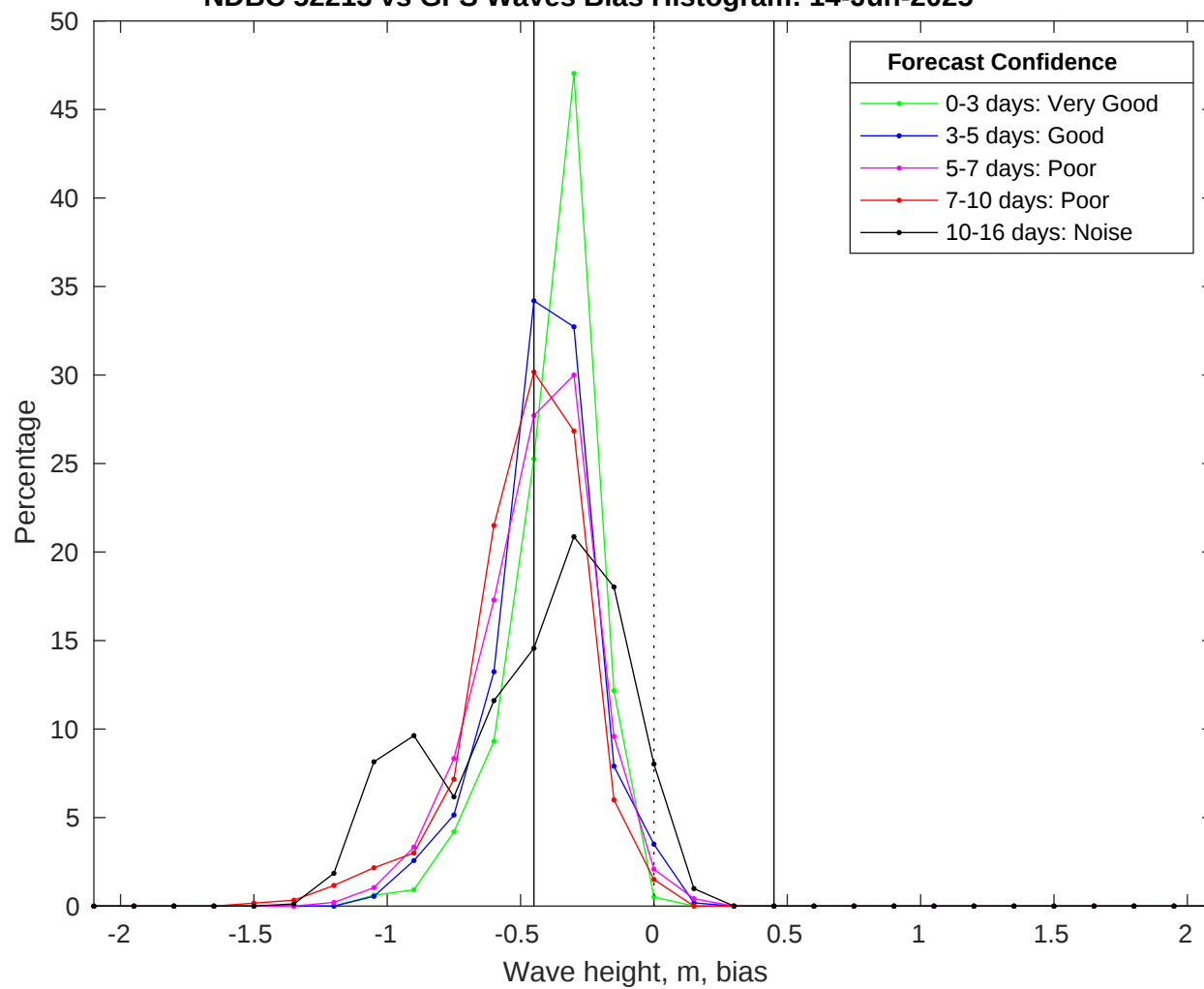
NDBC 52213 vs GFS Waves Bias Histogram: 14-Jun-2025
