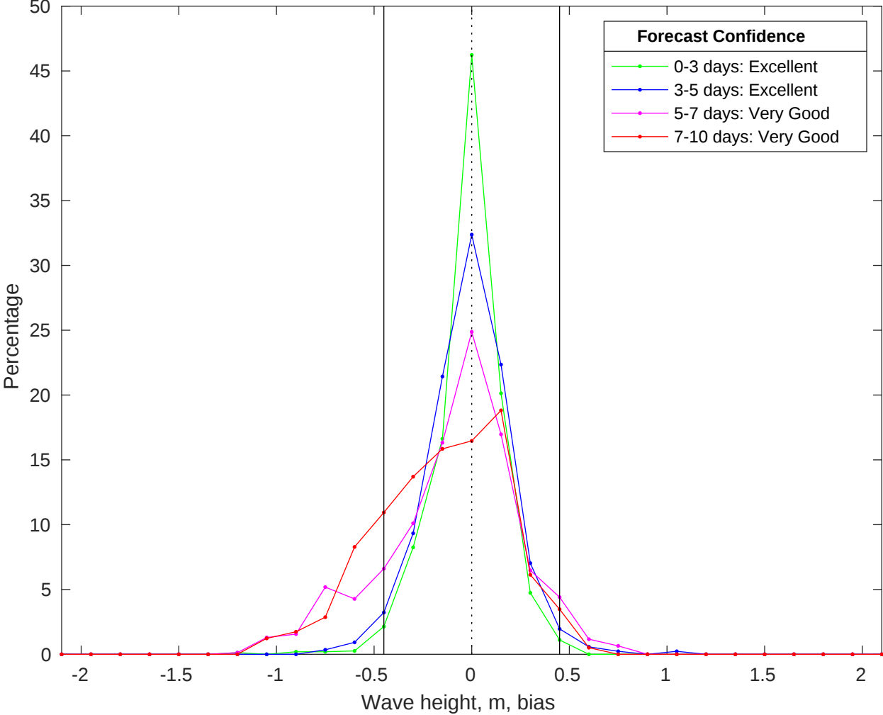
NDBC 41004 vs CMEMS Waves Bias Histogram: 15-Jun-2025
