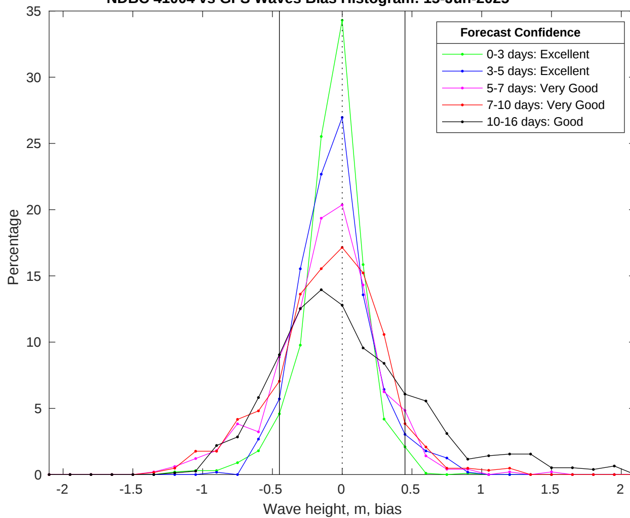
NDBC 41004 vs GFS Waves Bias Histogram: 15-Jun-2025
