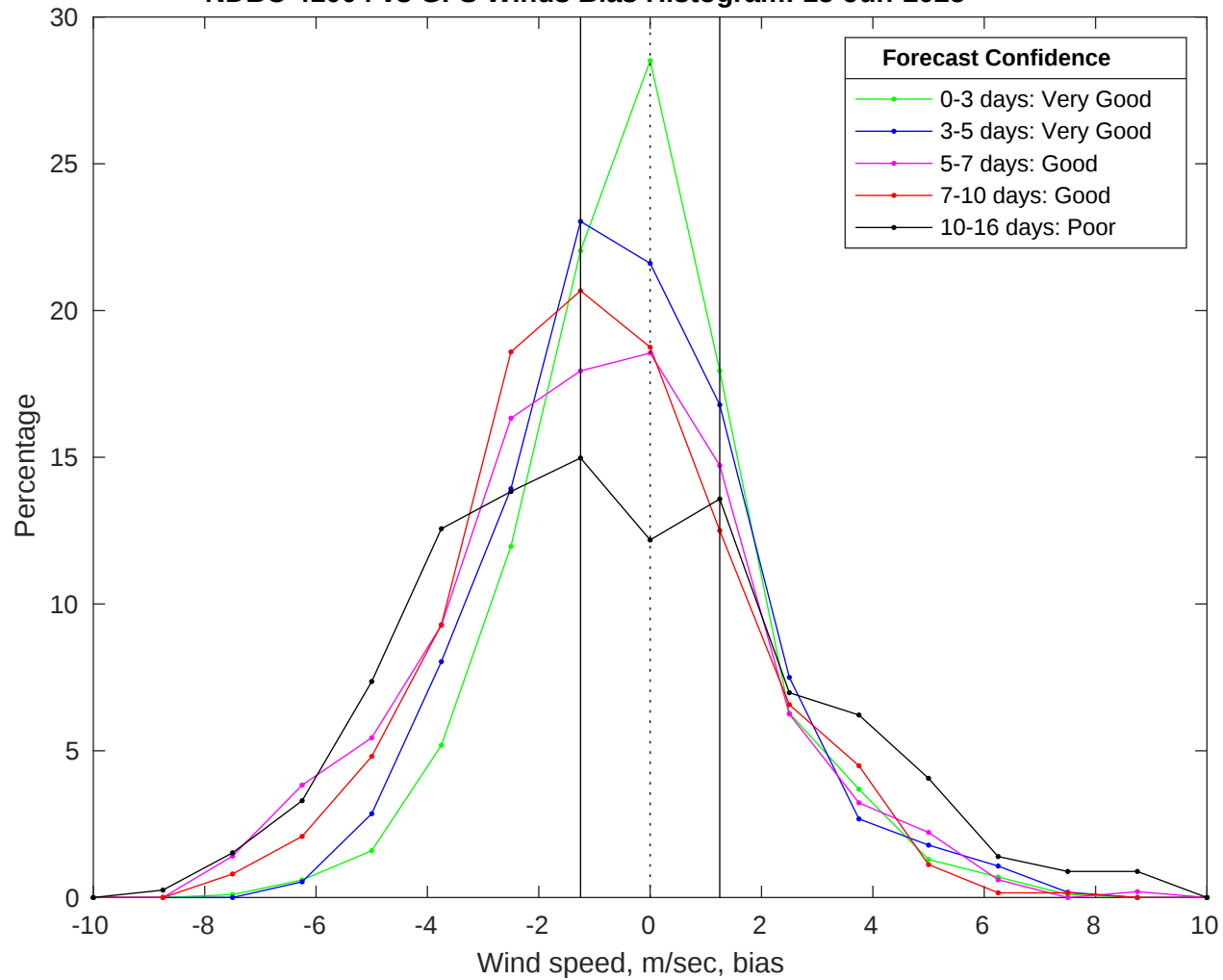
NDBC 41004 vs GFS Winds Bias Histogram: 15-Jun-2025
