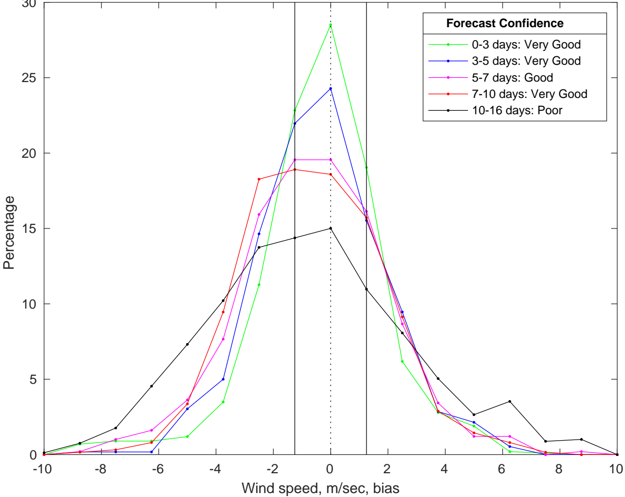
NDBC 41013 vs GFS Winds Bias Histogram: 15-Jun-2025
