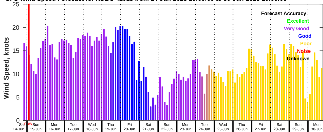
GFS Wind Speed Forecast for NDBC 41013 from 14-Jun-2025 19:00:00 to 30-Jun-2025 19:00:00
