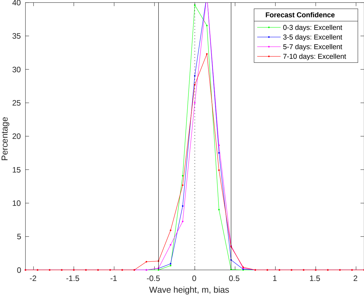
NDBC 41040 vs CMEMS Waves Bias Histogram: 15-Jun-2025
