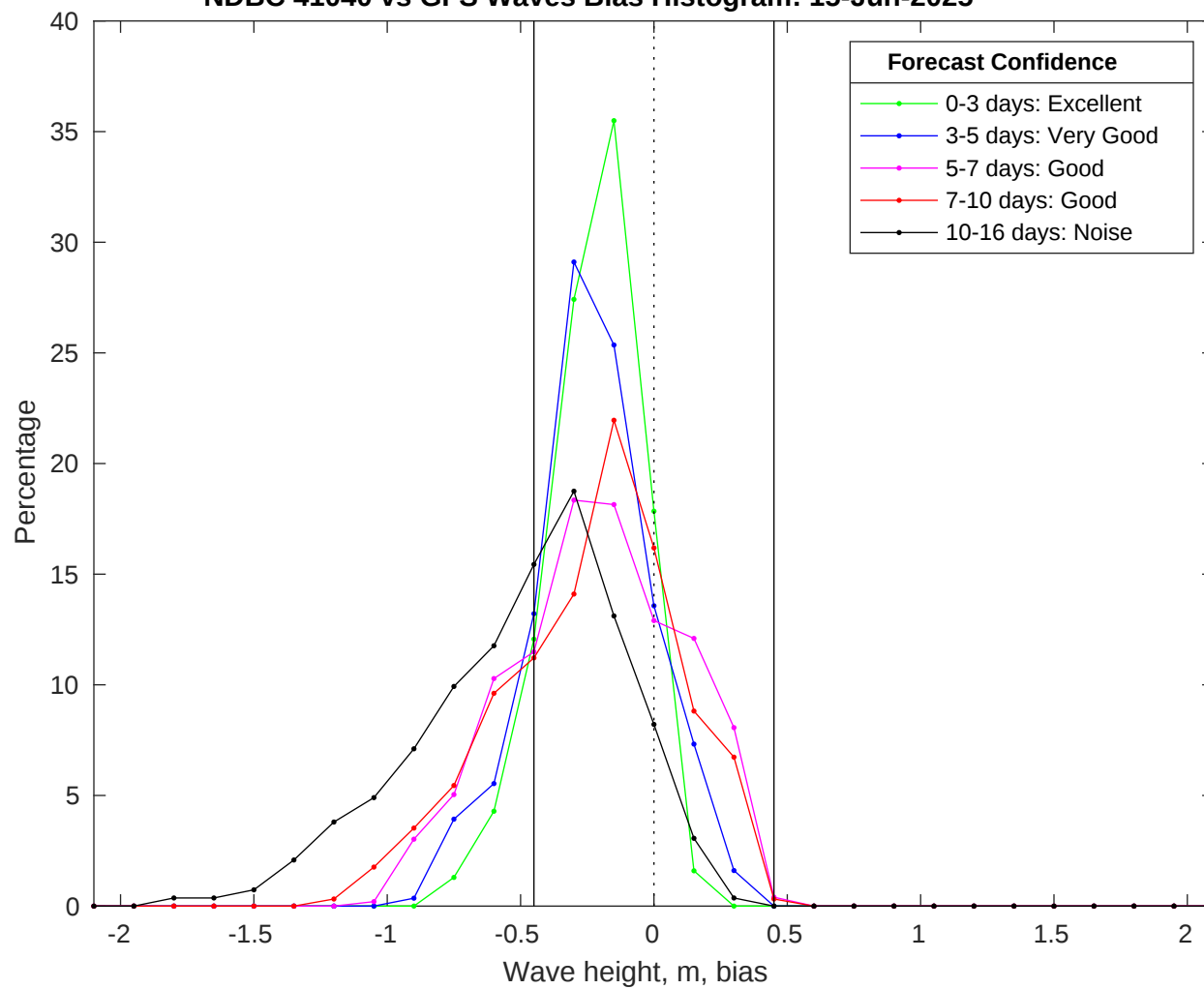
NDBC 41040 vs GFS Waves Bias Histogram: 15-Jun-2025
