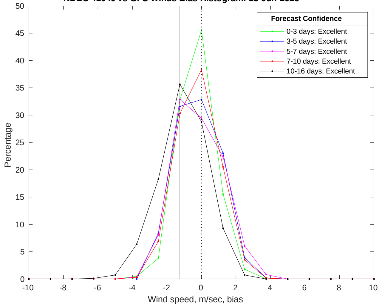
NDBC 41040 vs GFS Winds Bias Histogram: 15-Jun-2025
