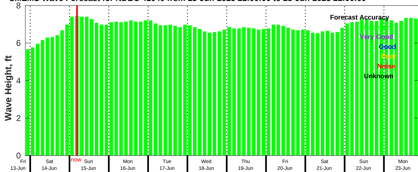
CMEMS Wave Forecast for NDBC 41040 from 13-Jun-2025 21:00:00 to 23-Jun-2025 21:00:00
