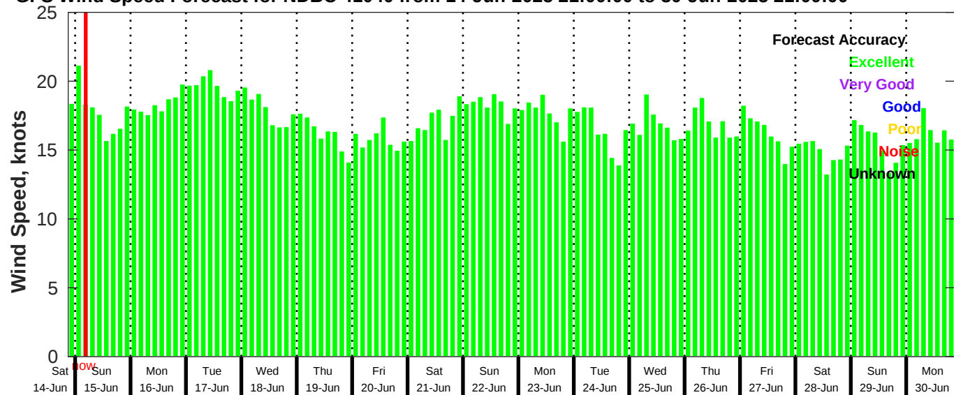
GFS Wind Speed Forecast for NDBC 41040 from 14-Jun-2025 21:00:00 to 30-Jun-2025 21:00:00
