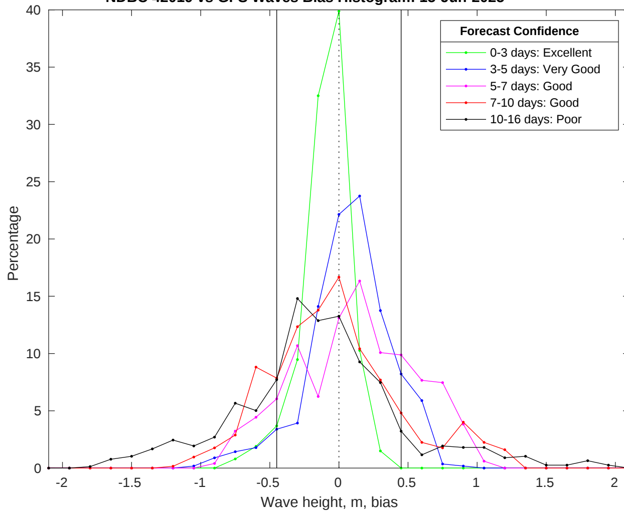
NDBC 42019 vs GFS Waves Bias Histogram: 15-Jun-2025
