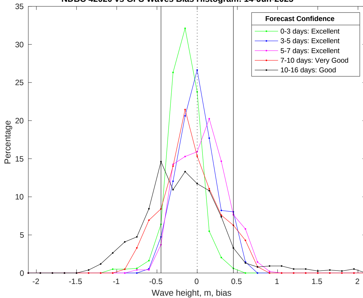
NDBC 42020 vs GFS Waves Bias Histogram: 14-Jun-2025
