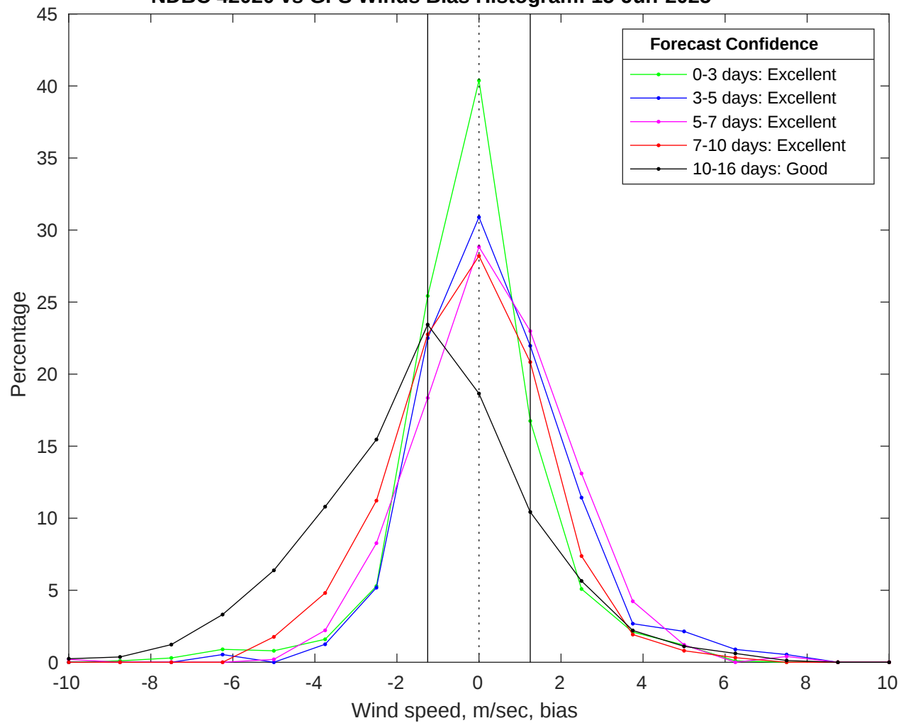
NDBC 42020 vs GFS Winds Bias Histogram: 15-Jun-2025
