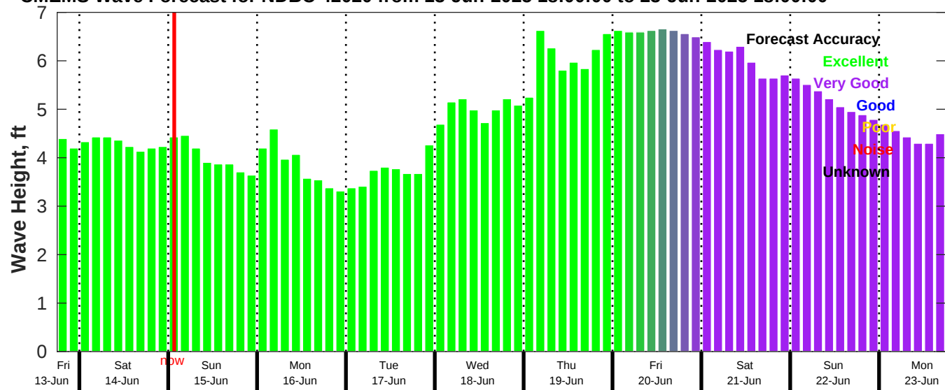
CMEMS Wave Forecast for NDBC 42020 from 13-Jun-2025 18:00:00 to 23-Jun-2025 18:00:00
