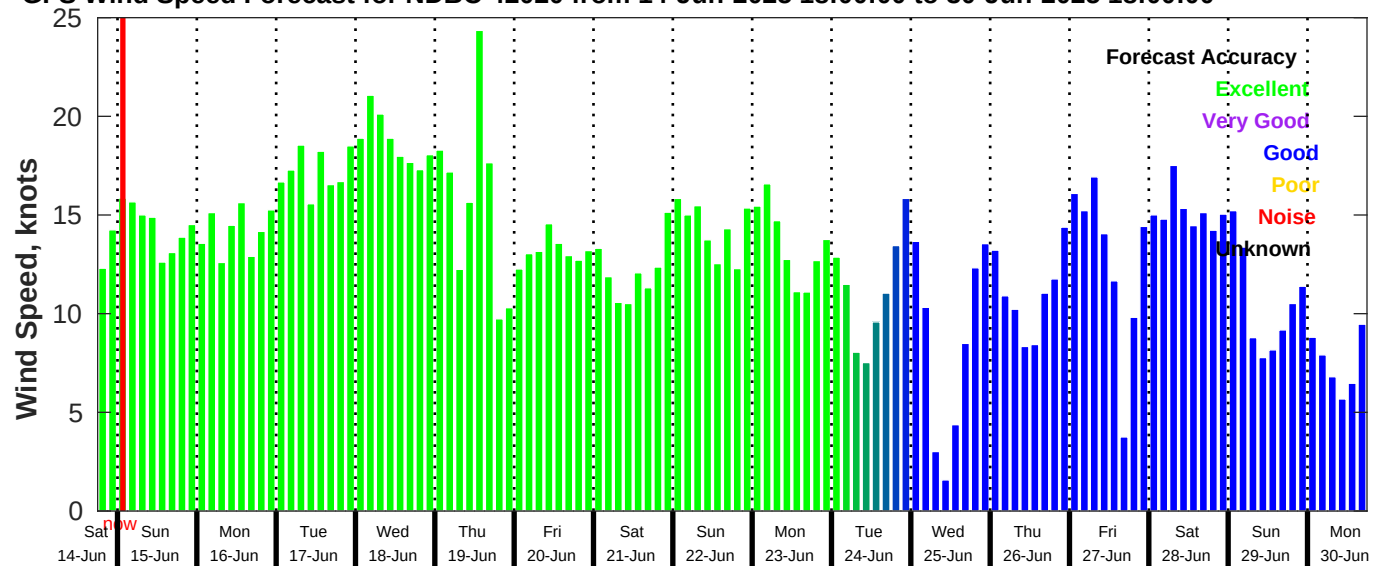
GFS Wind Speed Forecast for NDBC 42020 from 14-Jun-2025 18:00:00 to 30-Jun-2025 18:00:00
