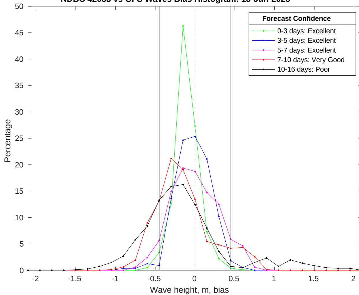
NDBC 42035 vs GFS Waves Bias Histogram: 15-Jun-2025
