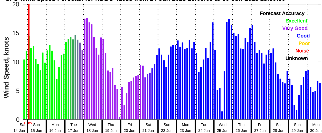
GFS Wind Speed Forecast for NDBC 42035 from 14-Jun-2025 18:00:00 to 30-Jun-2025 18:00:00
