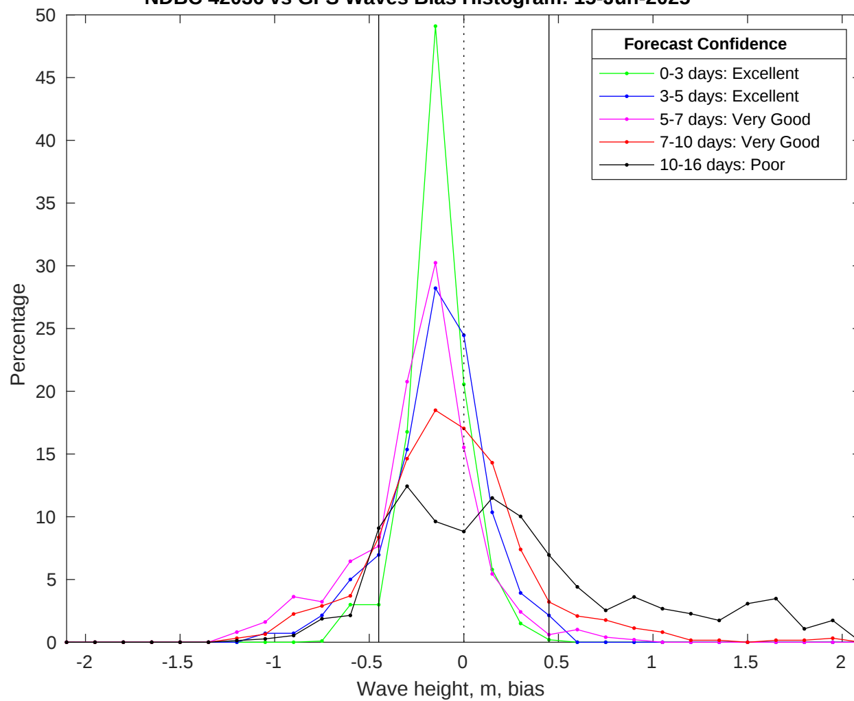
NDBC 42036 vs GFS Waves Bias Histogram: 15-Jun-2025
