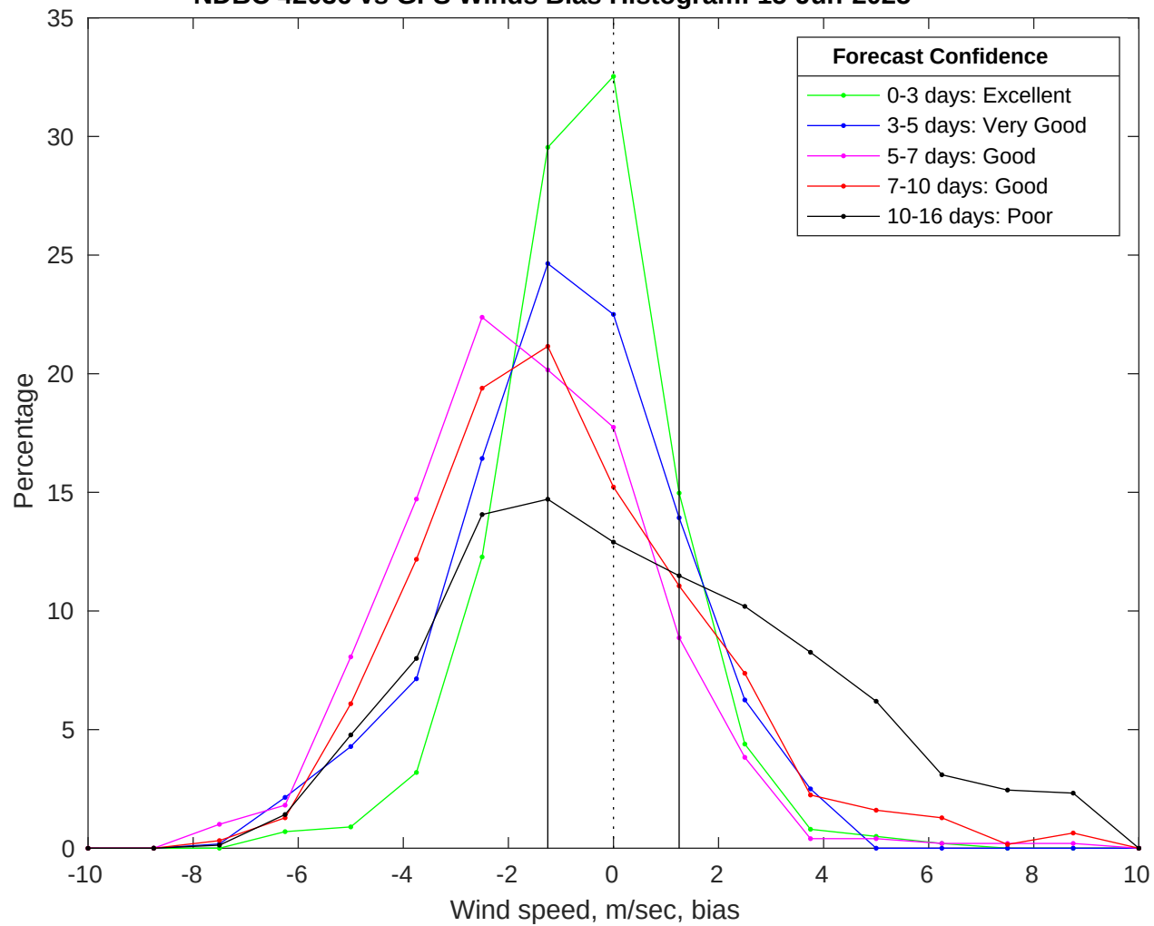
NDBC 42036 vs GFS Winds Bias Histogram: 15-Jun-2025
