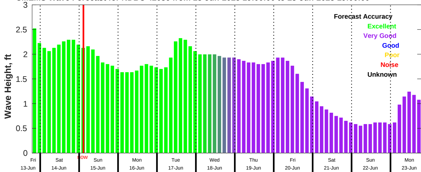
CMEMS Wave Forecast for NDBC 42036 from 13-Jun-2025 19:00:00 to 23-Jun-2025 19:00:00
