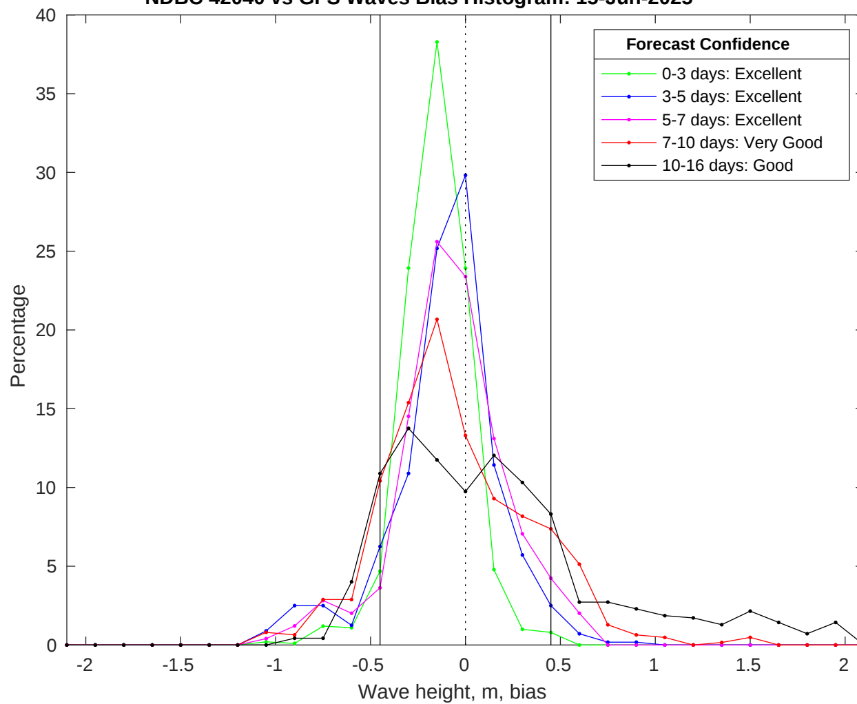
NDBC 42040 vs GFS Waves Bias Histogram: 15-Jun-2025
