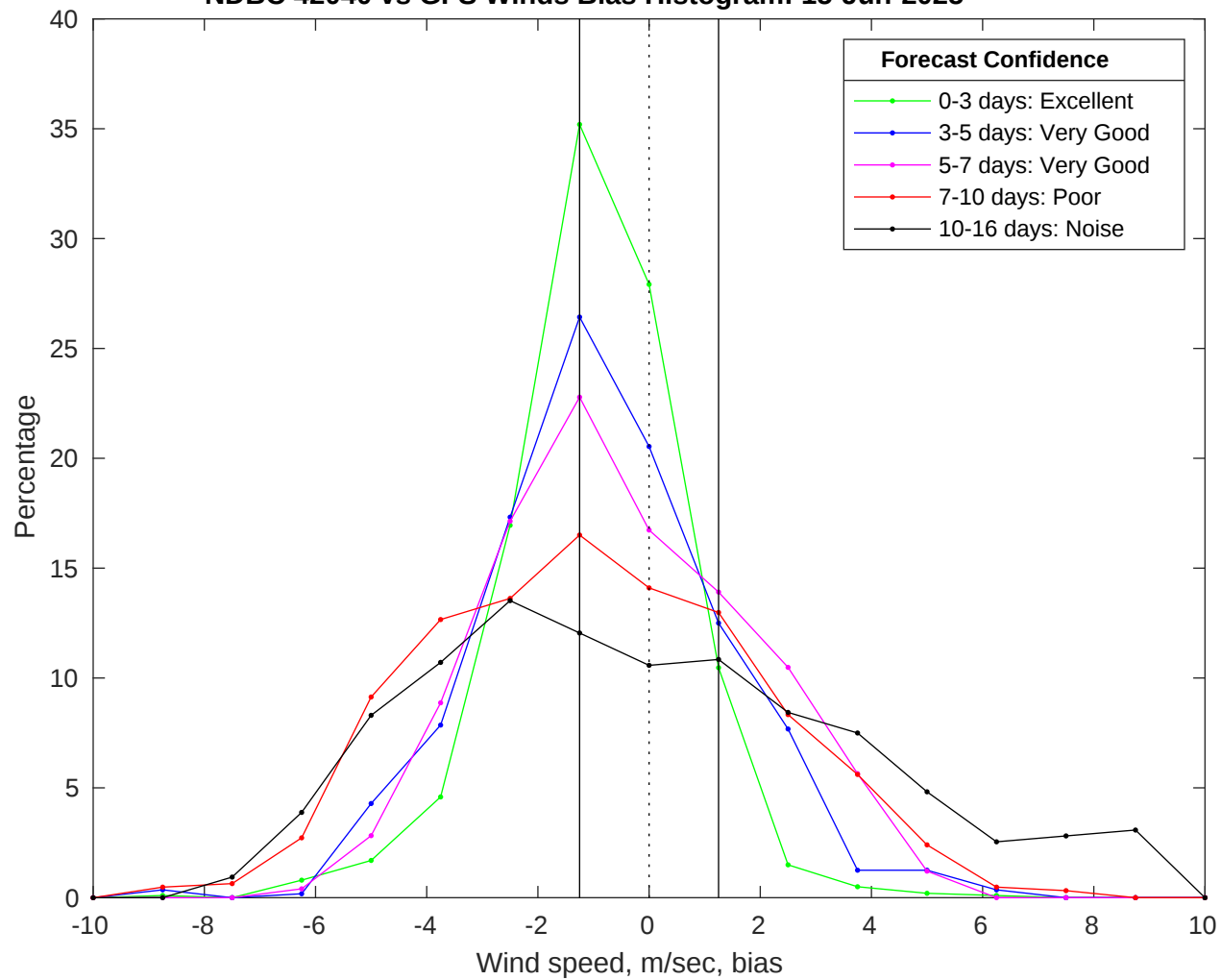
NDBC 42040 vs GFS Winds Bias Histogram: 15-Jun-2025
