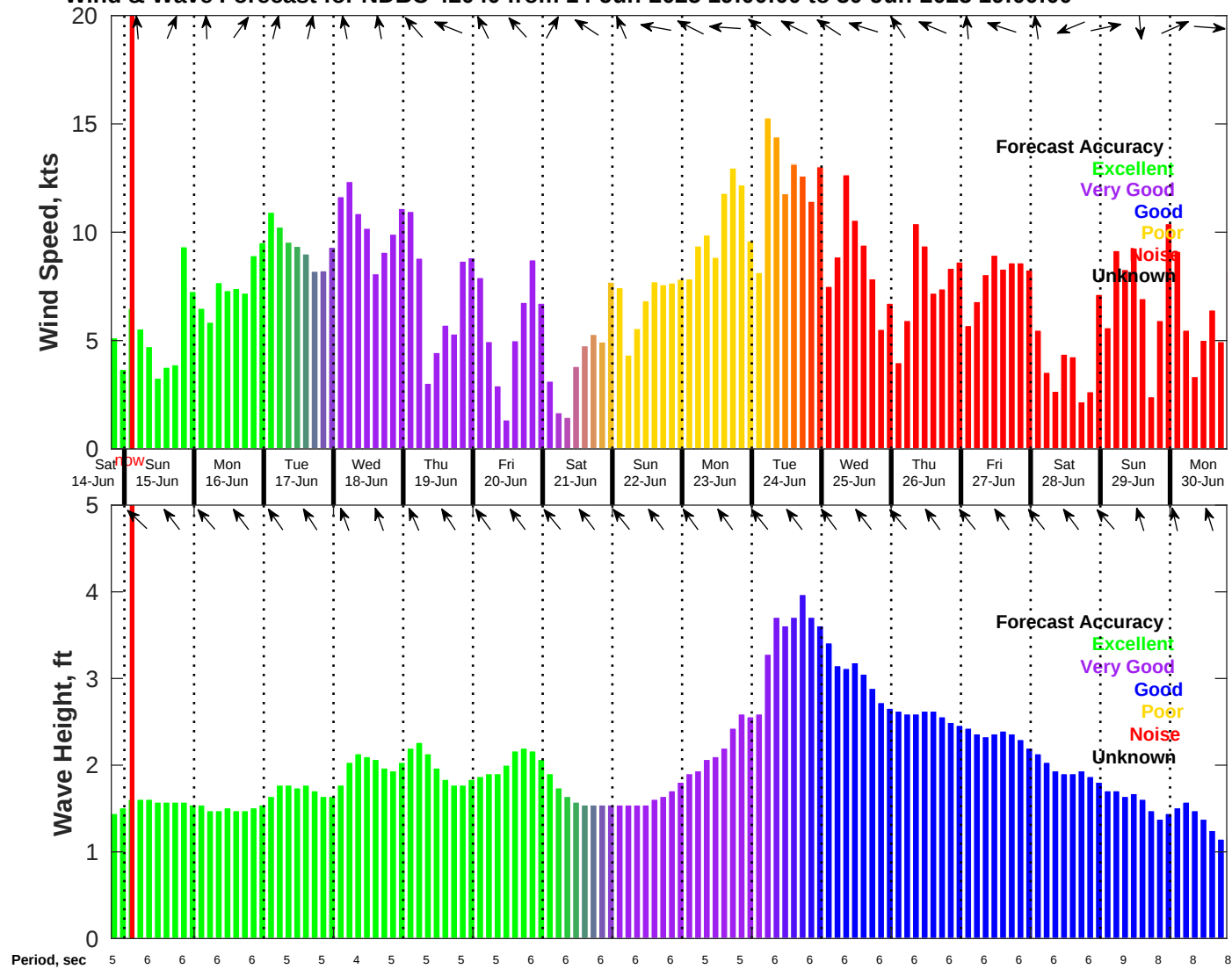
Wind & Wave Forecast for NDBC 42040 from 14-Jun-2025 19:00:00 to 30-Jun-2025 19:00:00
