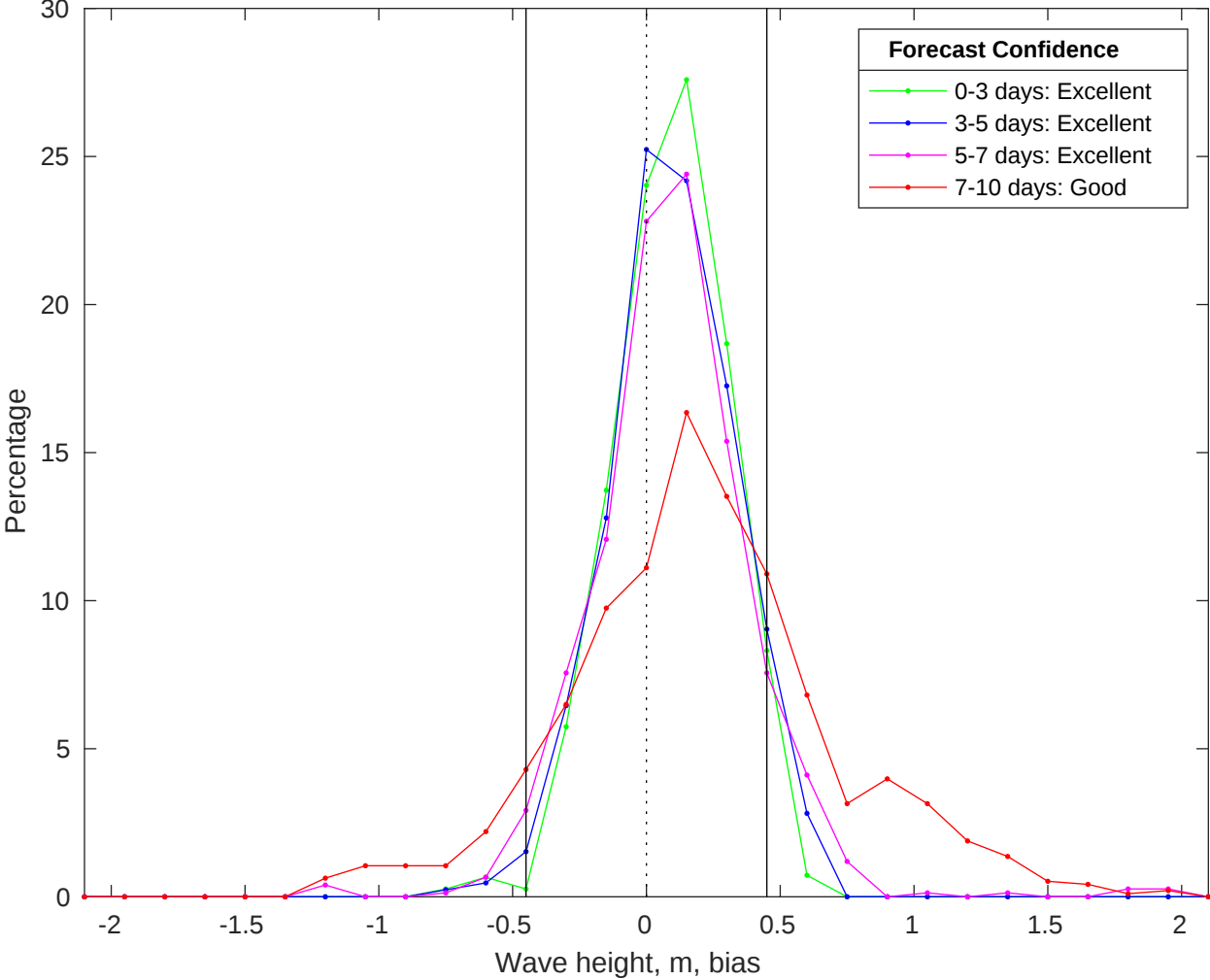
NDBC 46011 vs CMEMS Waves Bias Histogram: 15-Jun-2025
