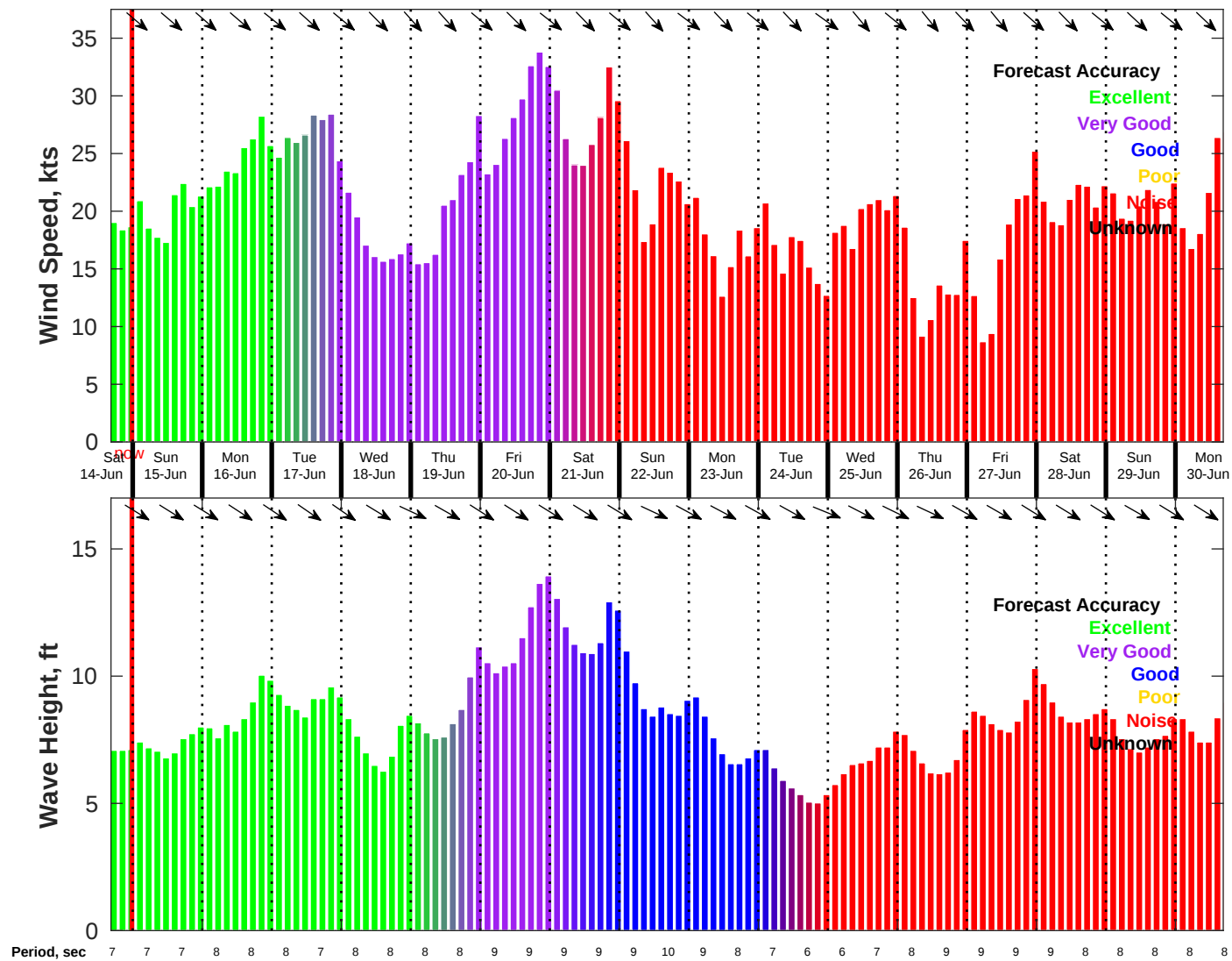
Wind & Wave Forecast for NDBC 46011 from 14-Jun-2025 16:00:00 to 30-Jun-2025 16:00:00
