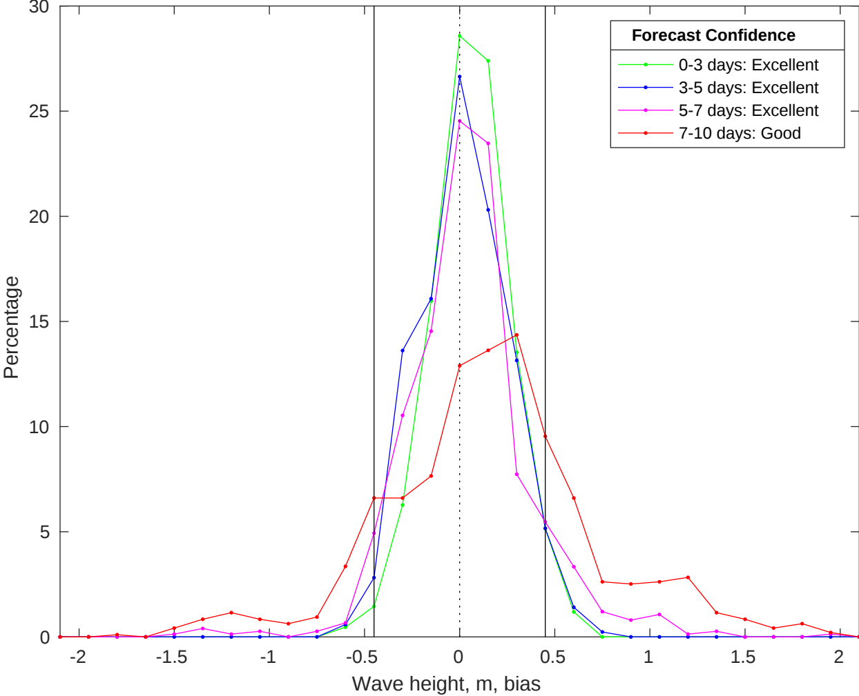
NDBC 46028 vs CMEMS Waves Bias Histogram: 15-Jun-2025
