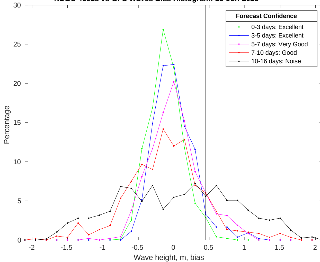
NDBC 46028 vs GFS Waves Bias Histogram: 15-Jun-2025
