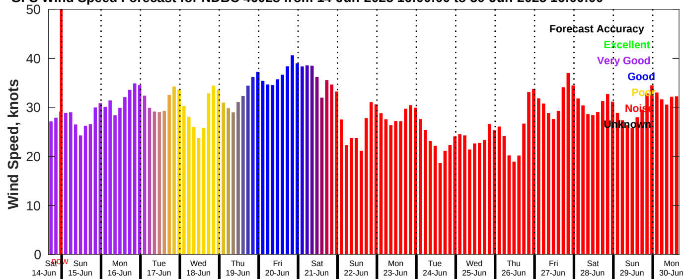
GFS Wind Speed Forecast for NDBC 46028 from 14-Jun-2025 16:00:00 to 30-Jun-2025 16:00:00
