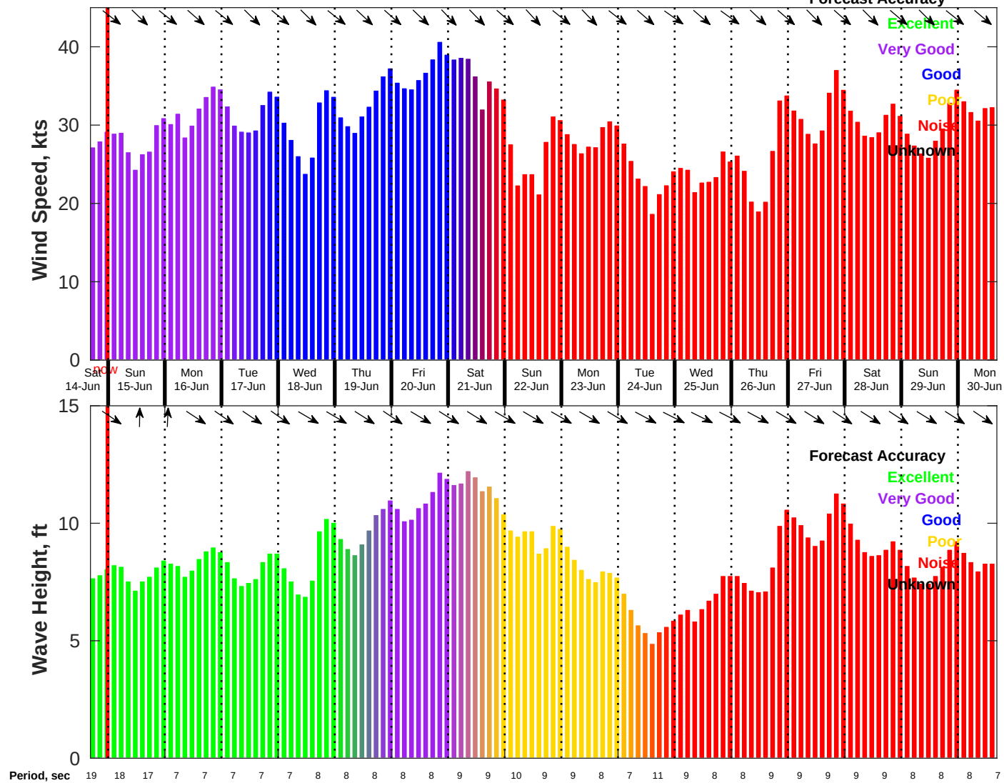
Wind & Wave Forecast for NDBC 46028 from 14-Jun-2025 16:00:00 to 30-Jun-2025 16:00:00
