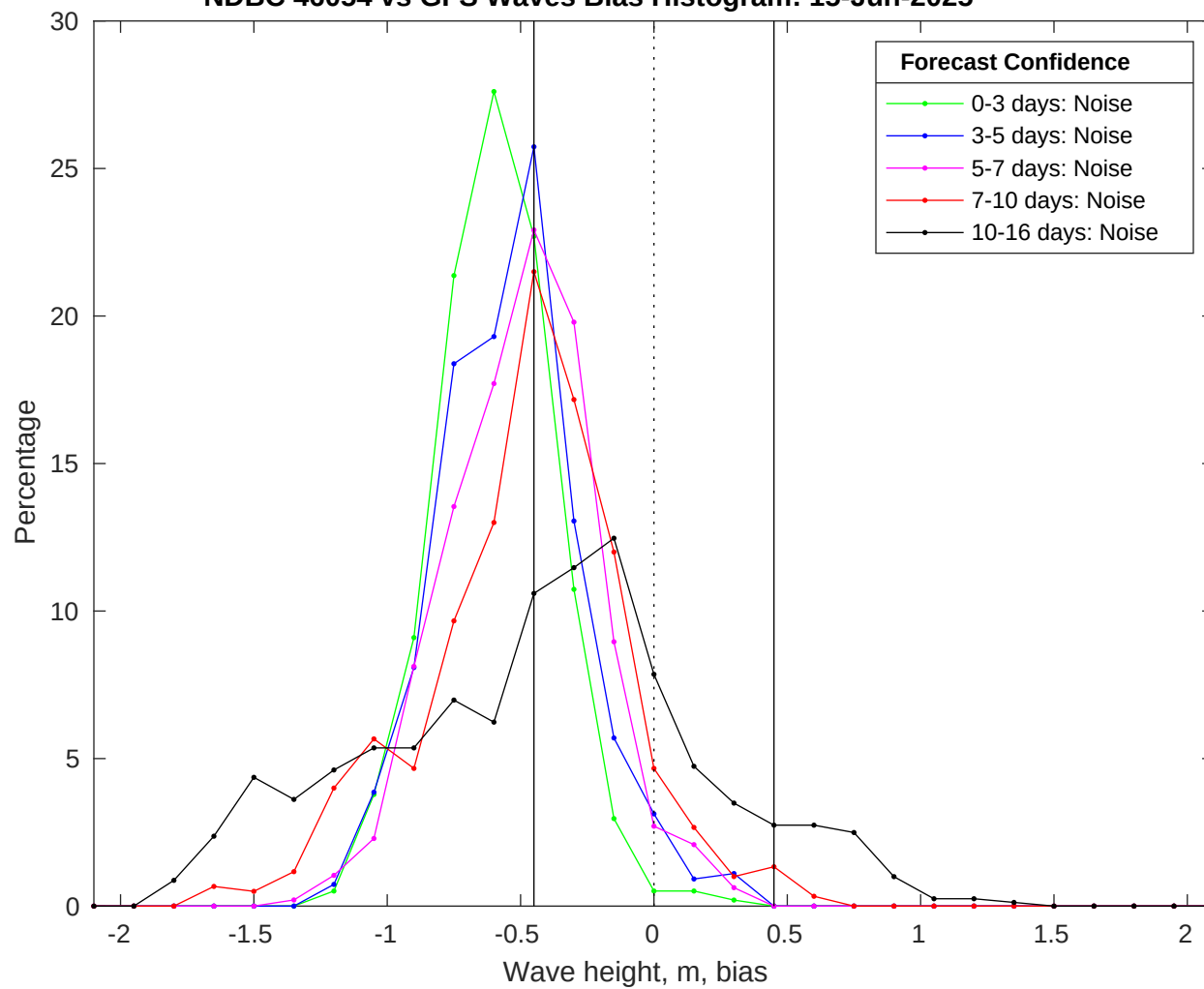
NDBC 46054 vs GFS Waves Bias Histogram: 15-Jun-2025
