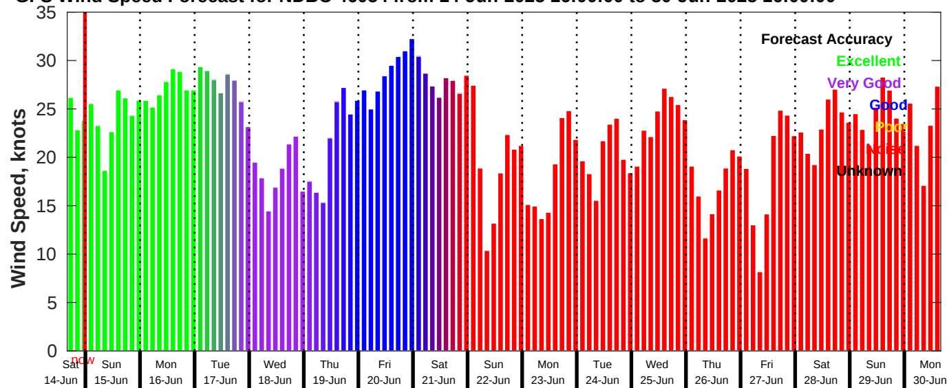
GFS Wind Speed Forecast for NDBC 46054 from 14-Jun-2025 16:00:00 to 30-Jun-2025 16:00:00
