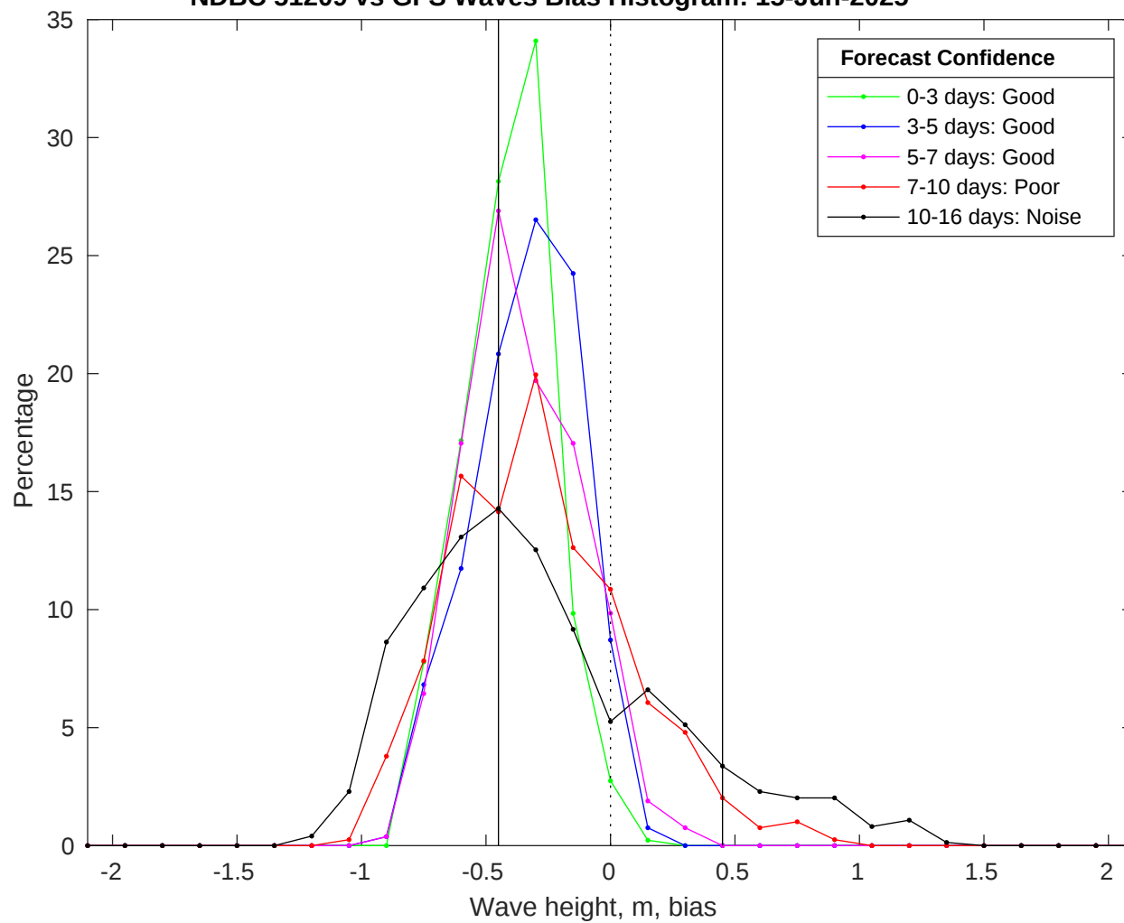
NDBC 51209 vs GFS Waves Bias Histogram: 15-Jun-2025
