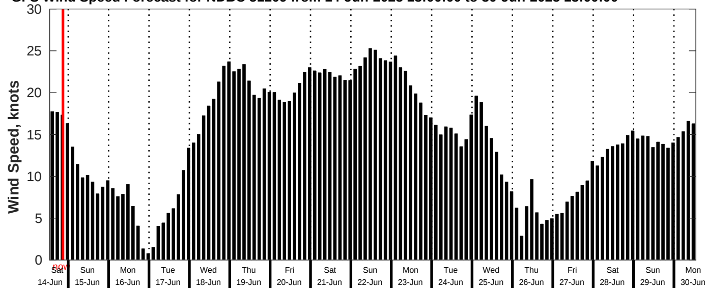
GFS Wind Speed Forecast for NDBC 51209 from 14-Jun-2025 13:00:00 to 30-Jun-2025 13:00:00
