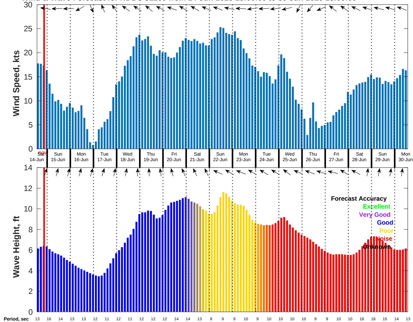
Wind & Wave Forecast for NDBC 51209 from 14-Jun-2025 13:00:00 to 30-Jun-2025 13:00:00
